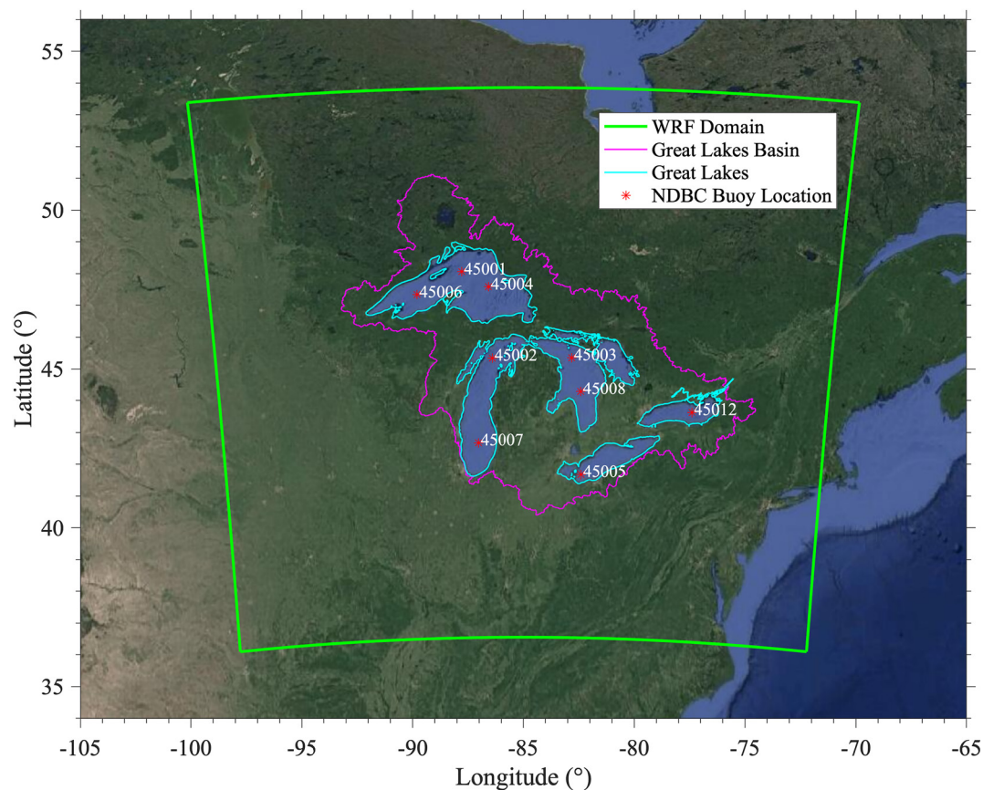
Figure 1. WRF's spatial domain (green) along with the outline for the Great Lakes Basin (magenta), the Great Lakes (cyan) and the locations for National Data Buoy Center (NDBC) buoys.
