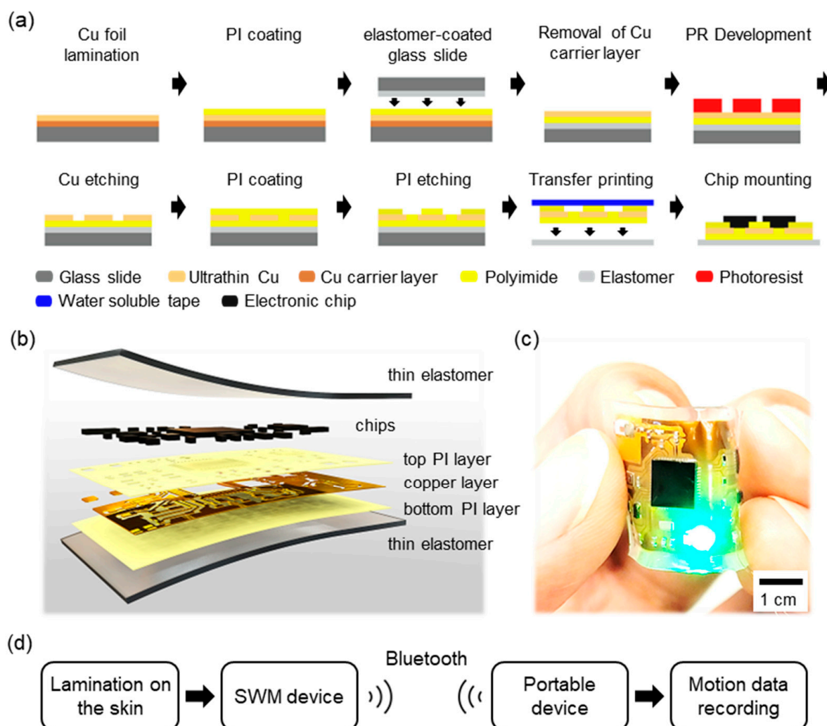
Figure 1. The overview of the skin-wearable device. (a) Illustration of device fabrication process using an ultrathin Cu film. (b) Exploded view of the device showing materials for each layer. (c) Device bending. (d) The flow of motion data from the skin to analysis.
