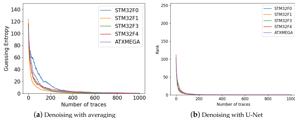
Figure 4. Comparison with different strategies for Gaussian noise removal of ASCAD dataset.
