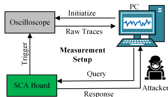
Figure 2. Overview of the SCA trace acquisition platform.
