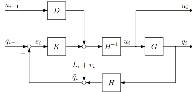
Figure 7. Block Diagram of CACC Controller
