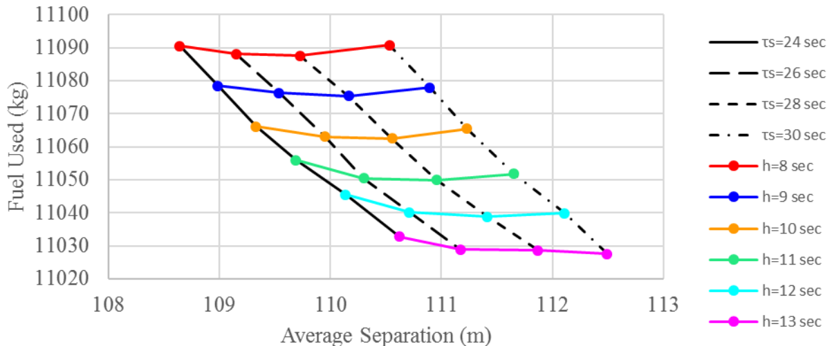
Figure 16. Average Separation and Fuel Consumption Tradeoff for KACC Controller
