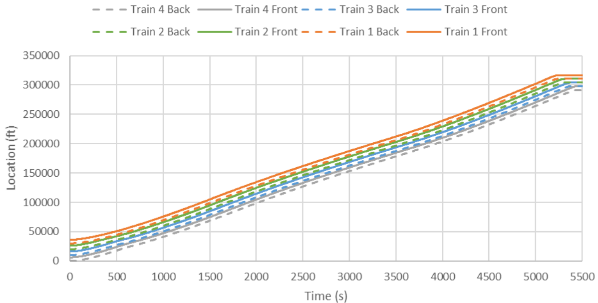
Figure 2. Stringline Diagram for Four-Train Baseline Simulation
