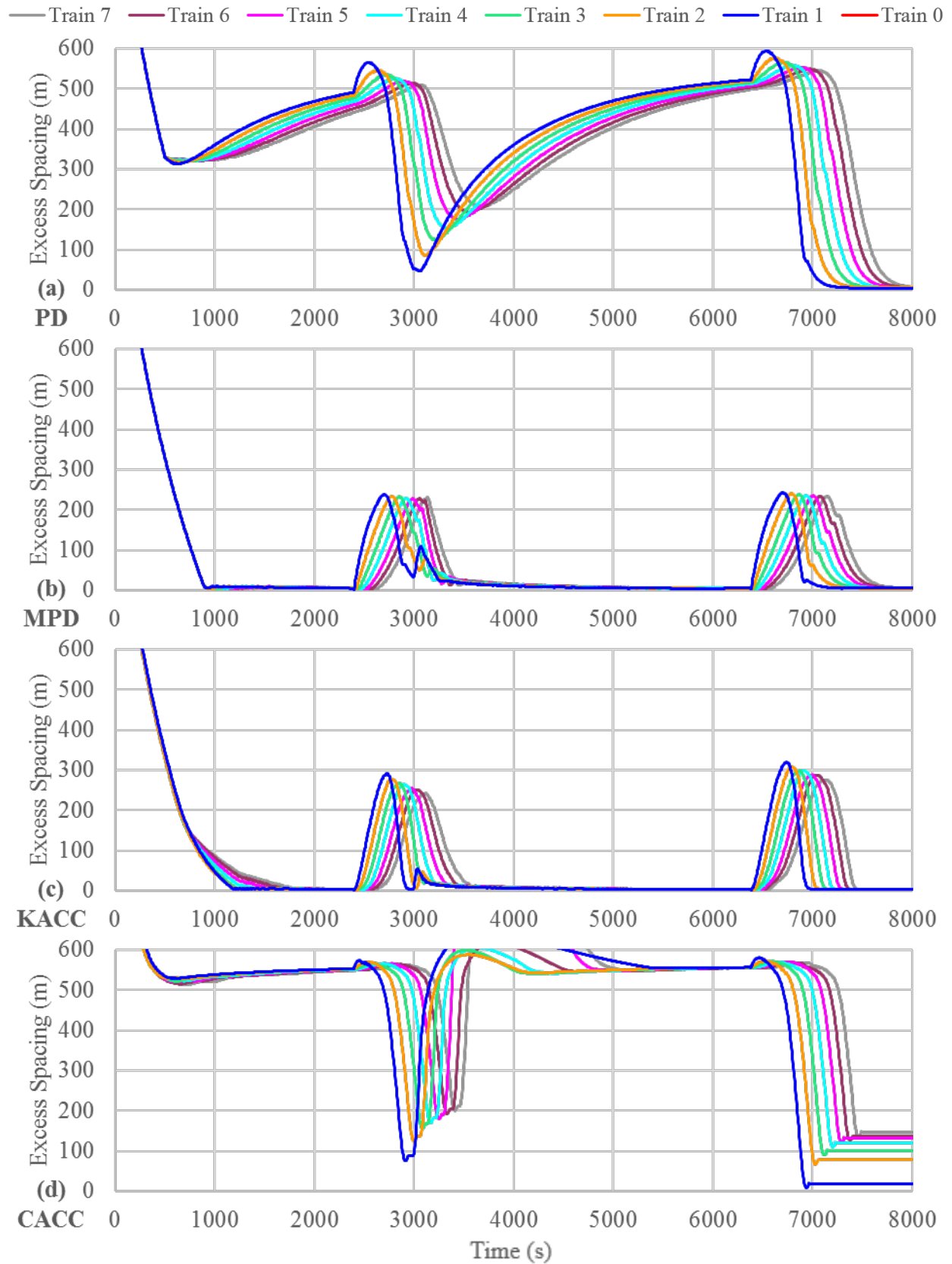
Figure 13. Position-Only Test Plan, Spacing Excess Comparison
