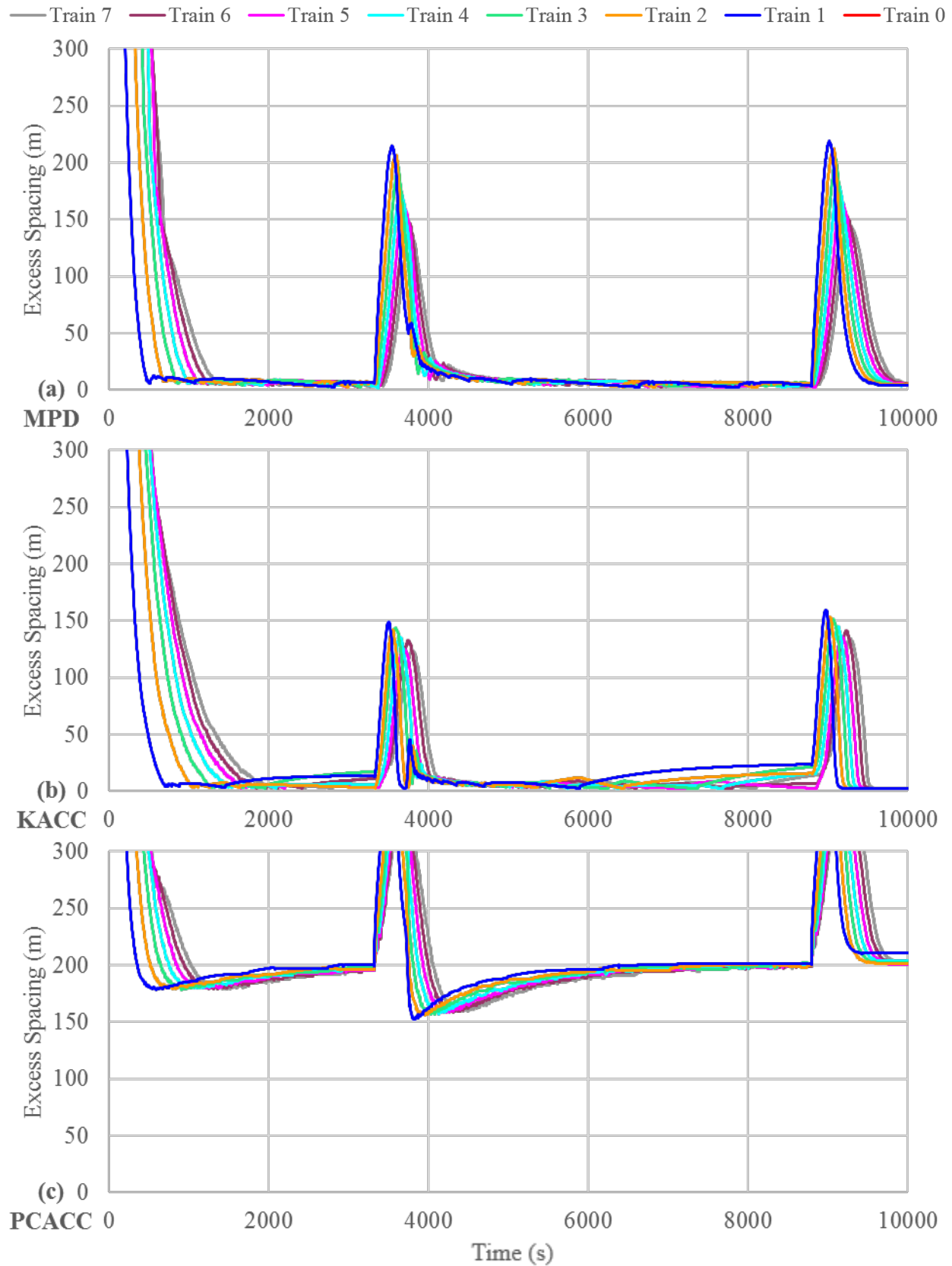
Figure 15. More Communication Test Plan, Spacing Excess Comparison
