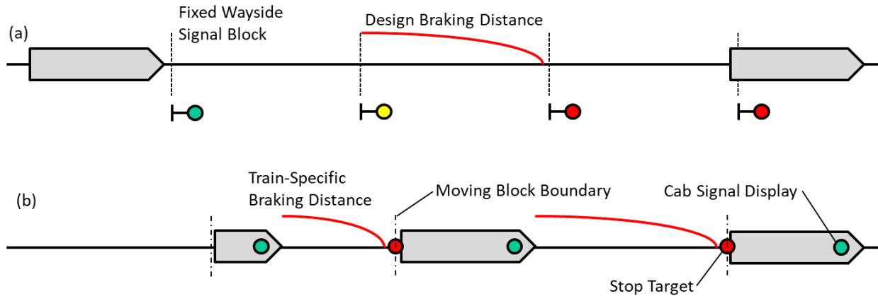
Figure 1. Train Operations and Headway Under a) Fixed Wayside Signal Blocks and b) Moving Blocks
