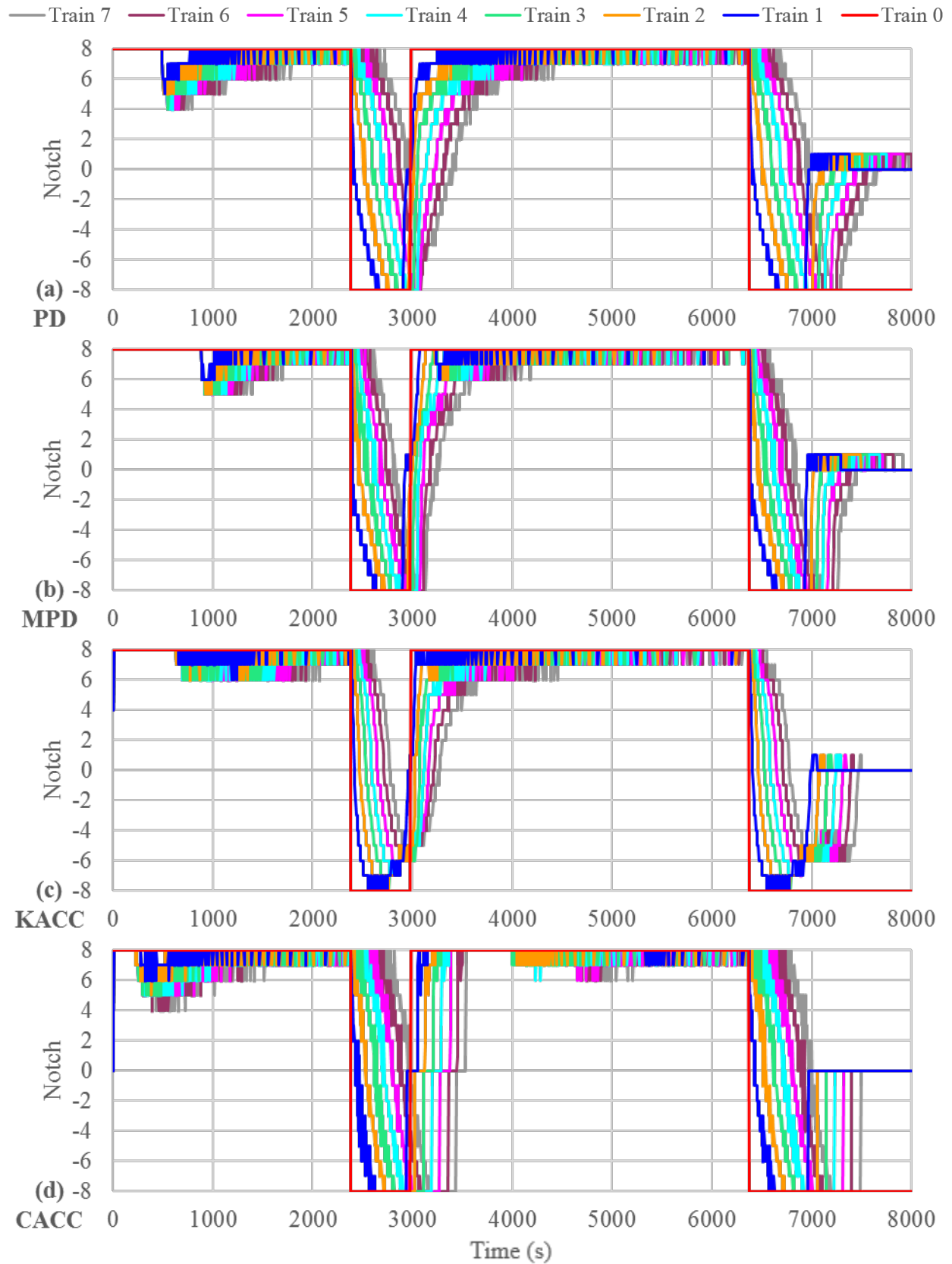
Figure 12. Position-Only Test Plan, Notch Performance Comparison
