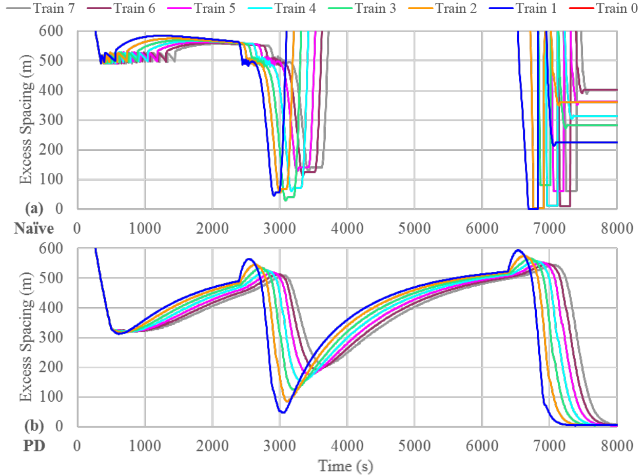
Figure 11. Naïve Controller versus PD Controller Excess Spacing
