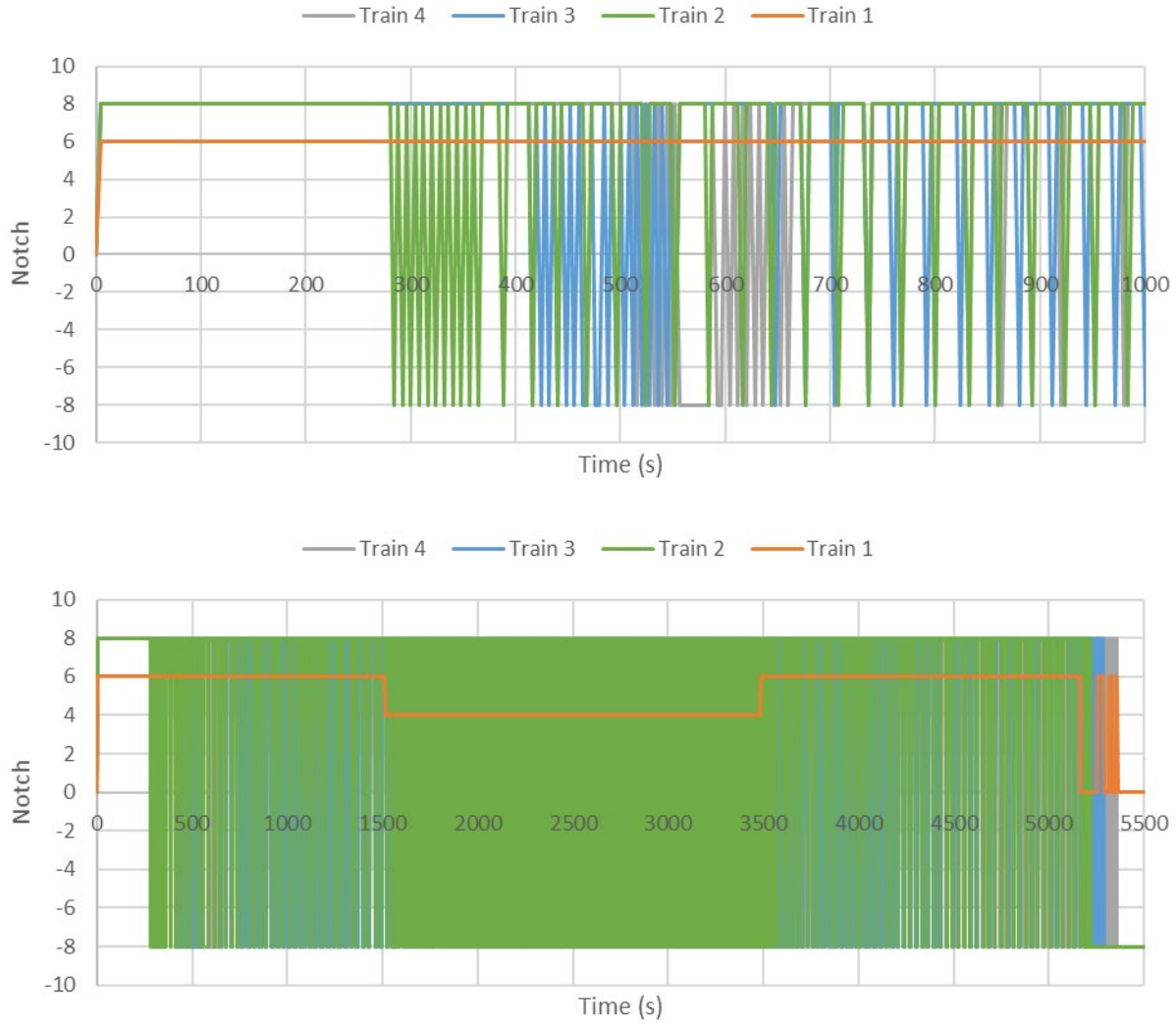
Figure 4. Throttle Notch Position for First 1,000 Seconds and Full Baseline Simulation
