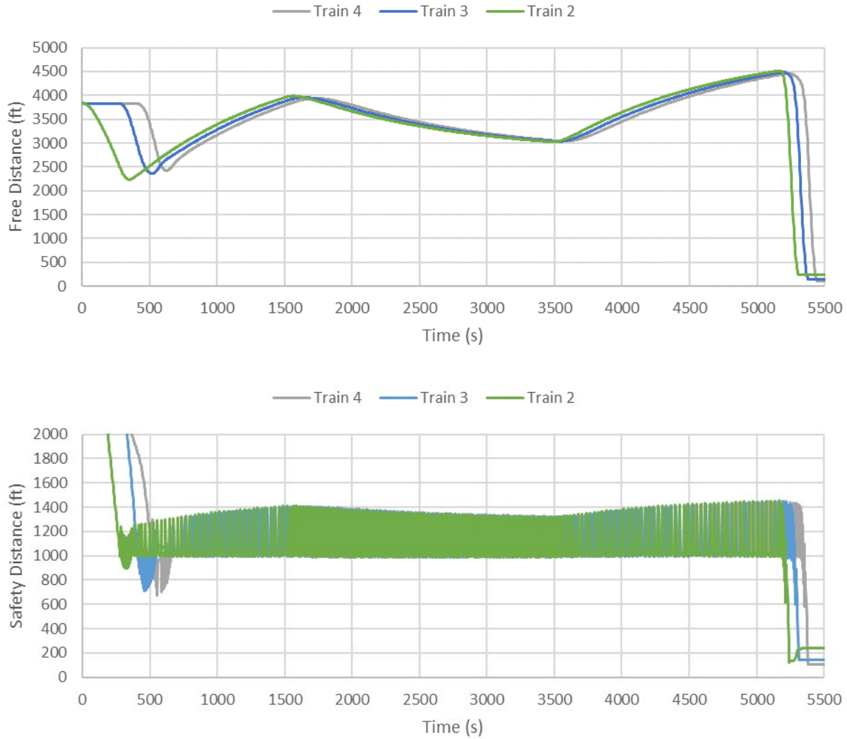
Figure 5. Train Spacing and Distance to PTC Enforcement for Baseline Simulation
