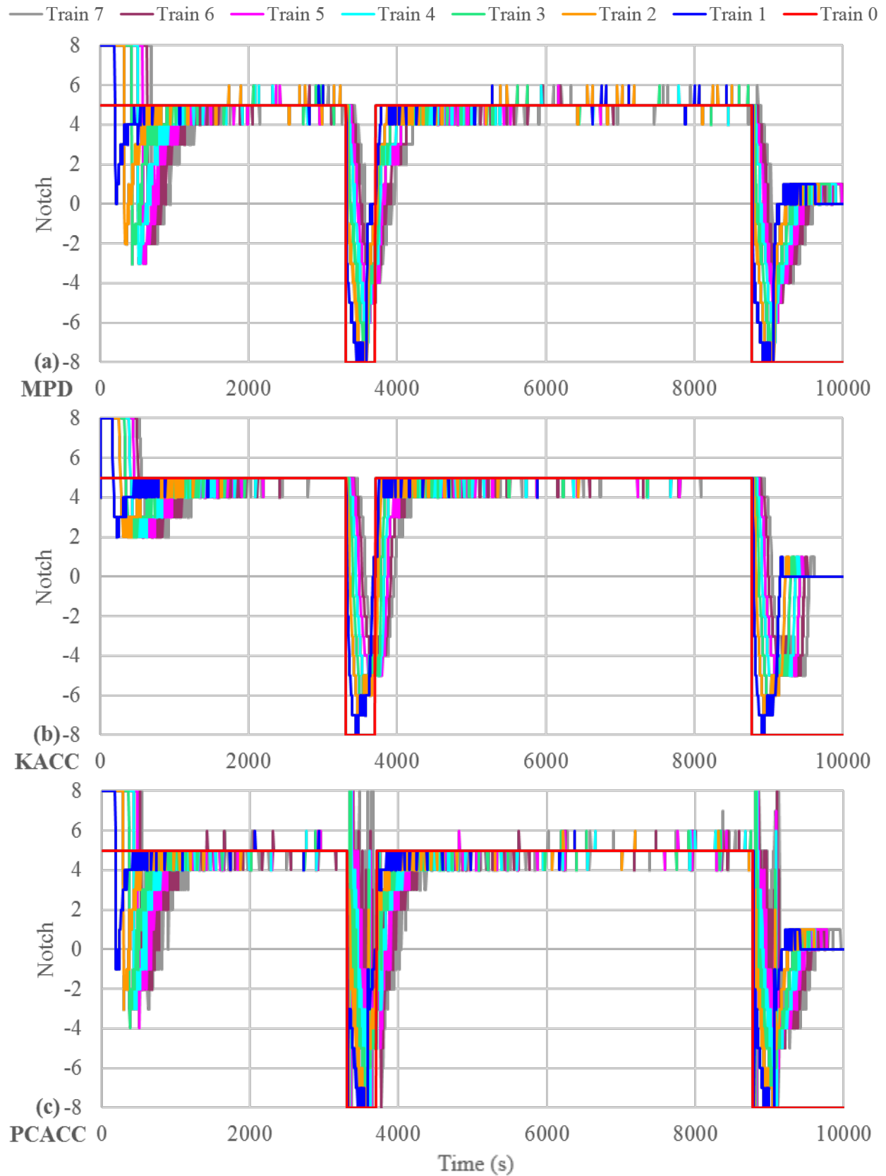
Figure 14. More Communication Test Plan, Notch Performance Comparison
