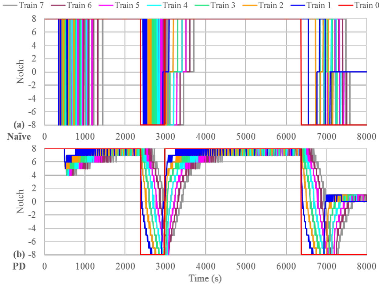
Figure 10. Naïve Controller versus PD Controller Notch Performance
