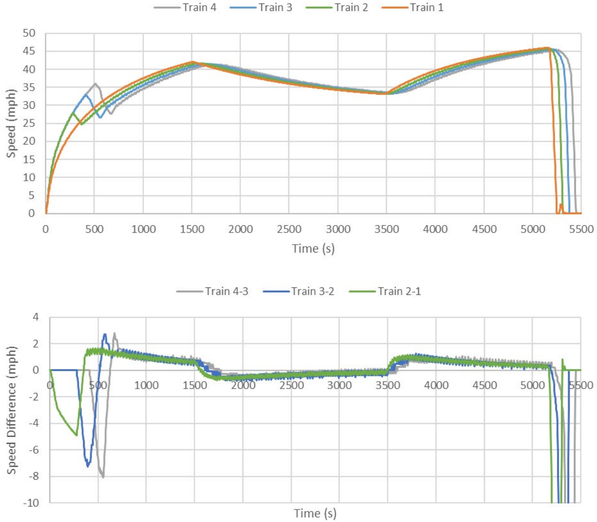
Figure 3. Absolute and Relative Train Speed over Time for Baseline Simulation
