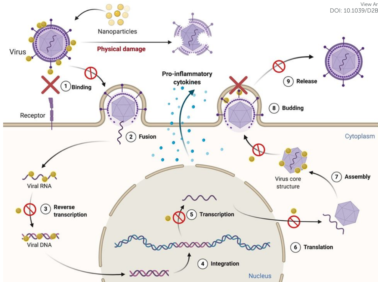
Figure 7. Schematic showing the mechanism of antiviral action of 0D nanoparticles.
