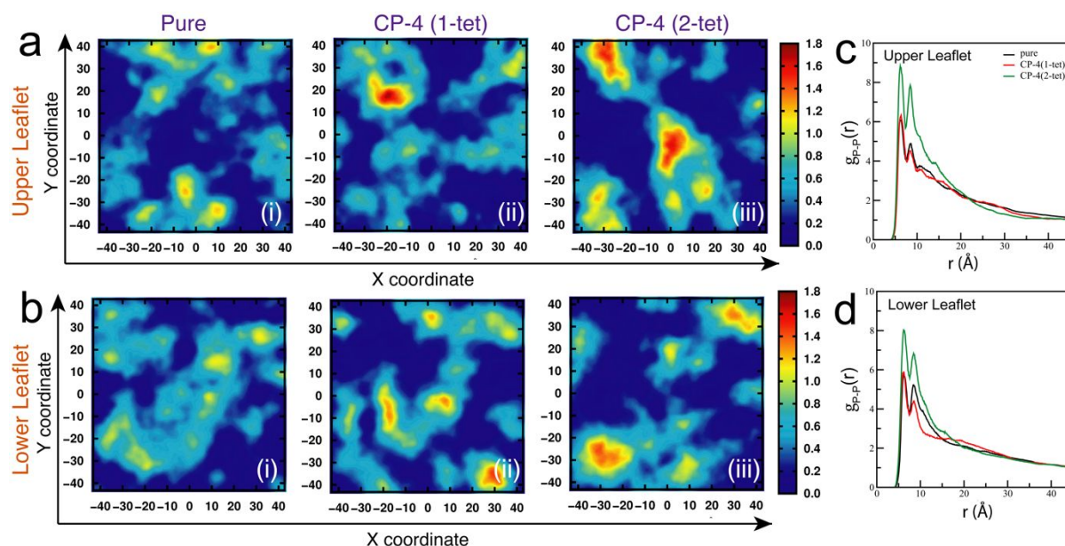
Figure 5: Anionic lipid clustering induced by quaternized pullulan. Two-dimensional number density plots for DOPG lipids in xy-plane orthogonal to membrane normal with subsequent addition of CP-4 molecules (a) upper leaflet & (b) lower leaflet. The units of x and y coordinates and number density are Å and Å -2 , respectively. Radial distribution function for P-P atomic pairs of DOPG lipid head groups for (c) upper leaflet (d) lower leaflet. Reproduced with permission 106 . Copyright 2022, Royal Society of Chemistry.
