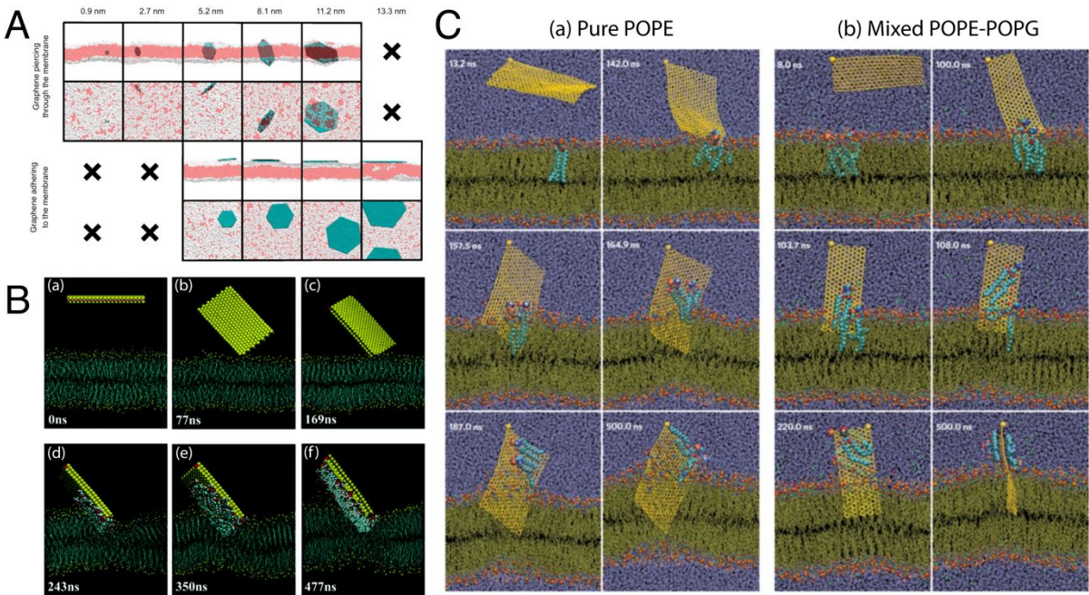
Figure 9: Mechanism of antibacterial action of 2-D nanosheets. A. Illustrative snapshots, at the end of the simulations, of six graphene nanosheets of increasing size. From left to right, sizes of 0.9, 2.7, 5.2, 8.1, 11.2, and 13.3 nm. White: hydrophilic heads of the phospholipids; red: hydrophobic phospholipid tails; petroleum blue: graphenes. For clarity, water is not shown. The top two rows are different perspectives of the six sheets, as are the bottom two rows. Only the five smaller sheets pierce through the membrane. The four larger sheets adhere to the membrane. Situations not observed in the simulations are indicated by “×”. Reproduced with permission 238 . Copyright 2015, American Chemical Society. B. Representative simulated trajectory of the restrictive simulation. (Snapshot time is shown in the lower left corner of each picture.) The MoS 2 nanosheet is shown as a yellow rectangular sandwich structure with S atoms
