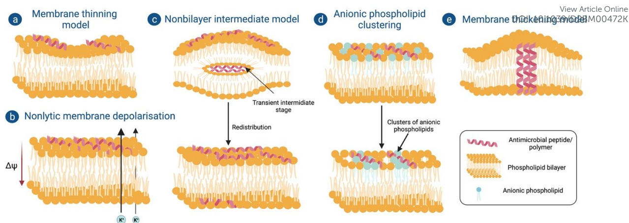
Figure 3. Schematic of different models showing “non-pore forming” mechanisms of membrane damage by antimicrobial macromolecules
