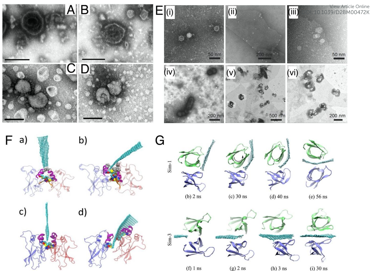
Figure 11. Mechanism of antiviral action of 2D nanosheets. Transmission electron microscopic images of GO-treated viruses. A. PRV control; B. PRV treated with GO for 1 h; C. PEDV control; and D. PEDV incubated with GO for 1 h. Scale bars: 200 nm (A, B) and 100 nm (C, D). Reproduced with permission 258 . Copyright 2015, American Chemical Society. E. TEM images of negative stained native EV71 (i) and GO captured EV71 complexes at (ii) low and (iii) high magnification; TEM images of negative stained (iv) H9N2 and GO captured H9N2 complexes at (v) low and (vi) high magnification with thermal heating treatment. Reproduced with permission 261 . Copyright 2015, Wiley. F. MD snapshots of the graphene insertion through the hexamer CTD-CTD interface. a–b) Initial breaking of A229/P234 and c–d) graphene disrupting the M241-I307 pair and inserting farther into the interface. Reproduced with permission 262 . Copyright 2017, Elsevier. G. Snapshots of the insertion process of a graphene sheet into the dimer. Reproduced with permission 263 . Copyright 2015, American Chemical Society.
