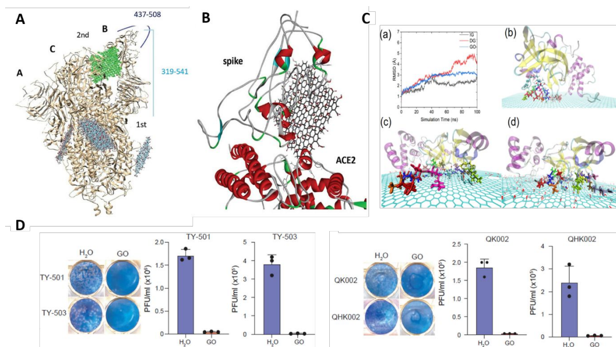
Figure 12: Anti-SARS-CoV-2 activity of 2D nanosheets. (A) Binding of GO at different sites of open state of spike protein (6VYB). (B) Binding of GO with spike-ACE2 complex (6M0J) with binding affinity -9.1 \text{ kcal mol}^{-1} . Reproduced with permission. Copyright 2021, Wiley. (C) Deactivation of the SARS-CoV-2 protease M pro by GO. (a) RMSD of the active pocket of M pro for all systems during 100 ns MD simulations. Representative snapshots of M pro adsorbed onto (b) IG, (c) DG, and (d) GO. Reproduced with permission. 265 Copyright 2021, American Chemical Society. (D) Anti-SARS-CoV-2 activity against Brazilian strains (TY7-501 and
