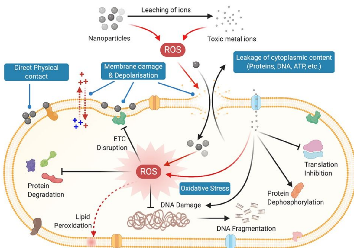
Figure 6. Schematic showing the mechanism of antibacterial action of 0D nanoparticles.
