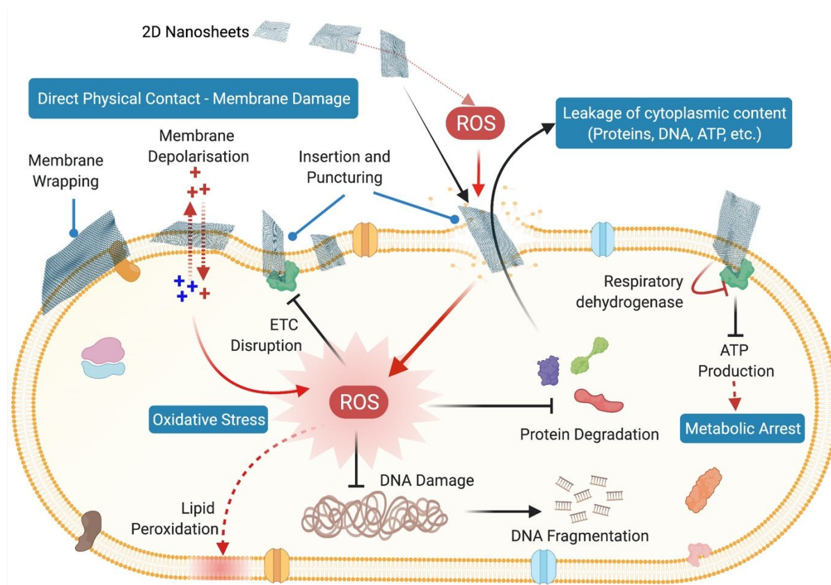
Figure 10. Schematic showing the mechanism of antibacterial action of 2D nanosheets
