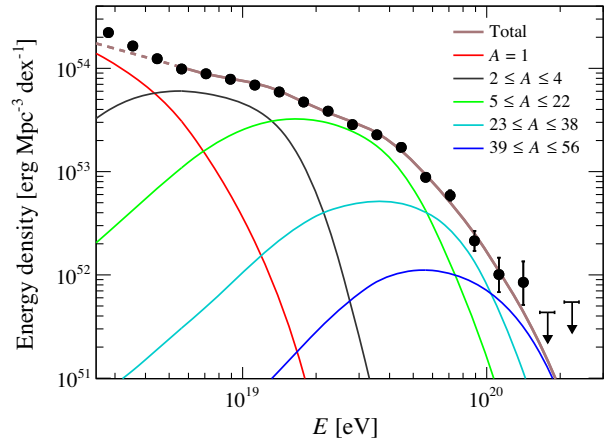
FIG. 2. Energy density obtained with the best fit parameters of the benchmark scenario used for illustration, as described in the text. The dashed curve shows the energy range that is not used in the fit and where an additional component is needed for describing the spectrum.
