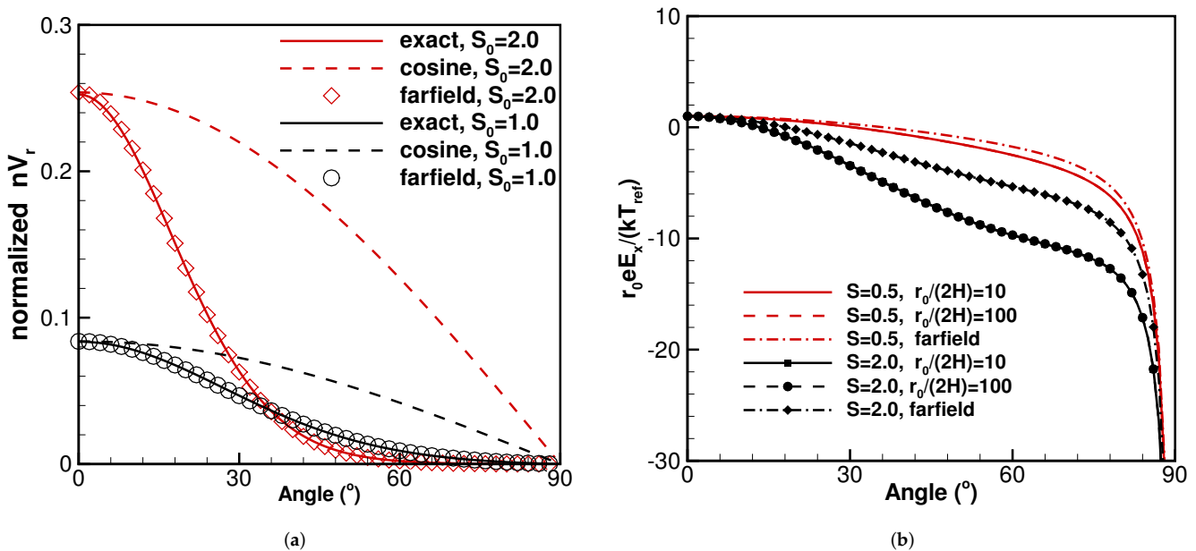
Figure 5. (a) Density flux profiles, r_0/(2H) = 10 ; (b) Normalized electric field component, r_0 E_x / (kT_0) , at different angles.
