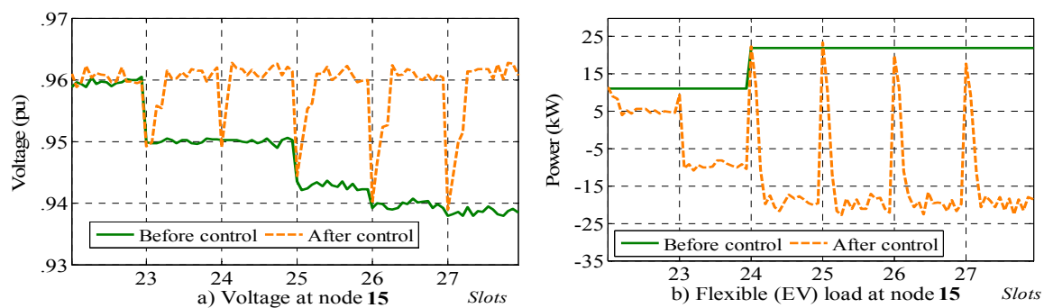
Figure 15. Adaptive variation of power per real-time monitored voltage.
