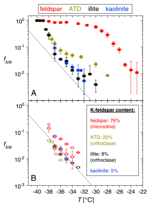
Figure 2. Measured ice fractions of feldspar (red) and illite-NX (black) as a function of temperature. Additionally, data from ATD (dark yellow) and Fluka kaolinite (blue) are shown. (a) Uncoated particles and (b) particles coated with sulfuric acid (circles: coating at 70°C; squares: coating at 80°C). Error bars are the standard deviation of the experiments and were obtained for temperatures with at least three measurements. For temperatures with fewer than three measurements, Poisson uncertainties are given. The gray line in both panels represents a fit curve through all the coated minerals (except the feldspar coated at 70°C) following the fit equation f_{ice} = 3E - 11 \cdot e^{-0.563 \cdot T} .
