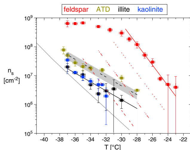
Figure 3. n_s values for the feldspar sample (red) and illite-NX (black) as a function of temperature. The straight lines are exponential fits to our data ( n_s = 0.0155 \cdot e^{-0.824 \cdot T} for feldspar and n_s = 37.066 \cdot e^{-0.353 \cdot T} for illite-NX). The dotted, the dash-dotted and the dashed red lines represent the n_s fits of feldspar lowered by a factor of 10, 100 and 1000, respectively. The gray shaded area shows the n_s -fit of illite-NX increased by a factor of 2 to 4. The black dashed line is the n_s of illite-NX increased by a factor of 3, which corresponds to a K-feldspar mass fraction of 8%, as given in Atkinson et al. [2013]. The gray line represents the baseline which we assume to represent clay minerals, without any K-feldspar. The fit equation of the gray line is n_s = 0.0029 \cdot e^{-0.606 \cdot T} .
