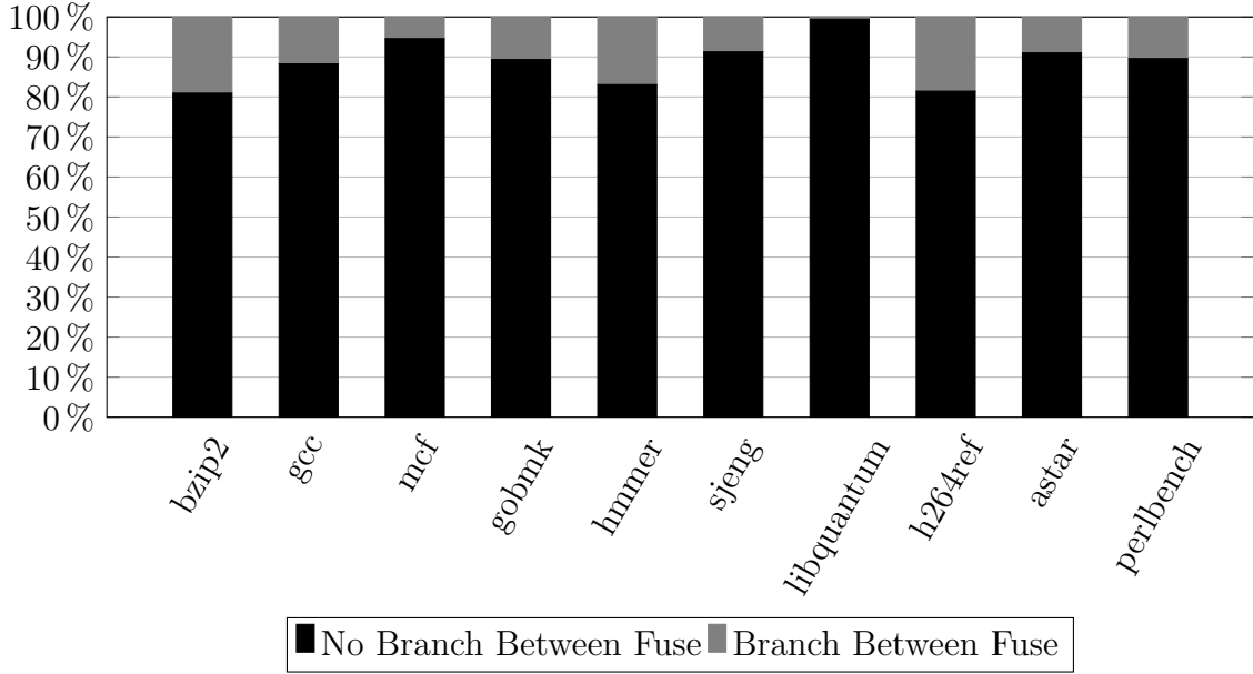
Figure 3.1: Branches Between Fusible Instructions[2]
