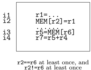
Figure 2.12: Memory Cloaking
