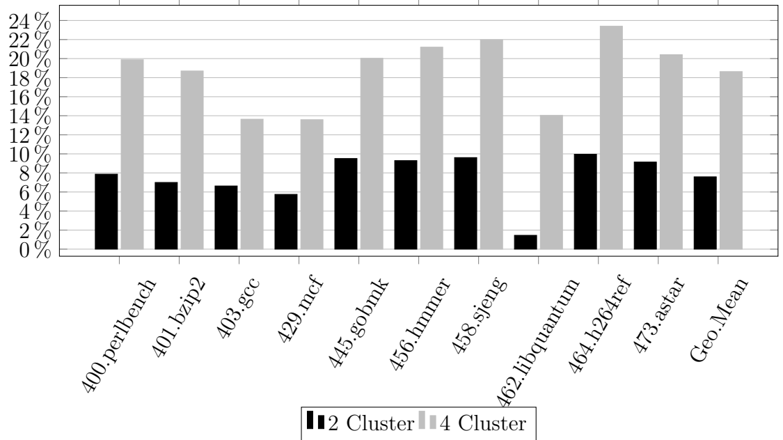
Figure 4.9: Generated Copy Instructions as a Percentage of Total
