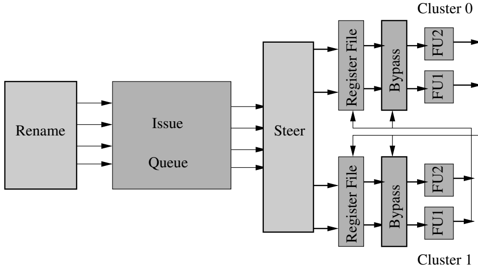
Figure 4.7: Unified window uni-directional two cluster architecture
