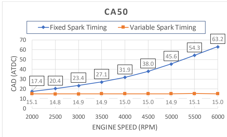
Figure 4.2: CA50 of fixed and variable spark timing
