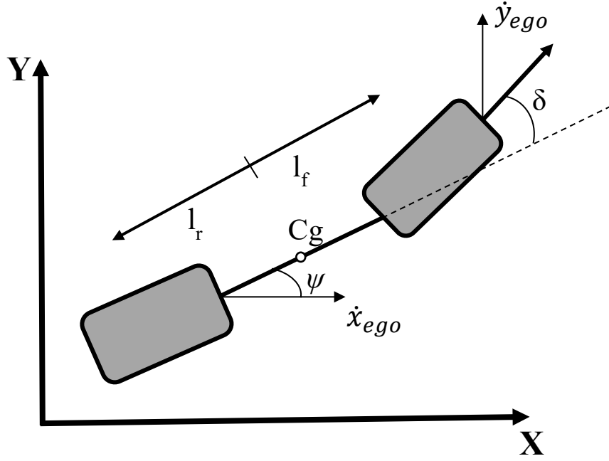
Figure 3.3: Representation of the dynamic bicycle model for lateral control [39]
