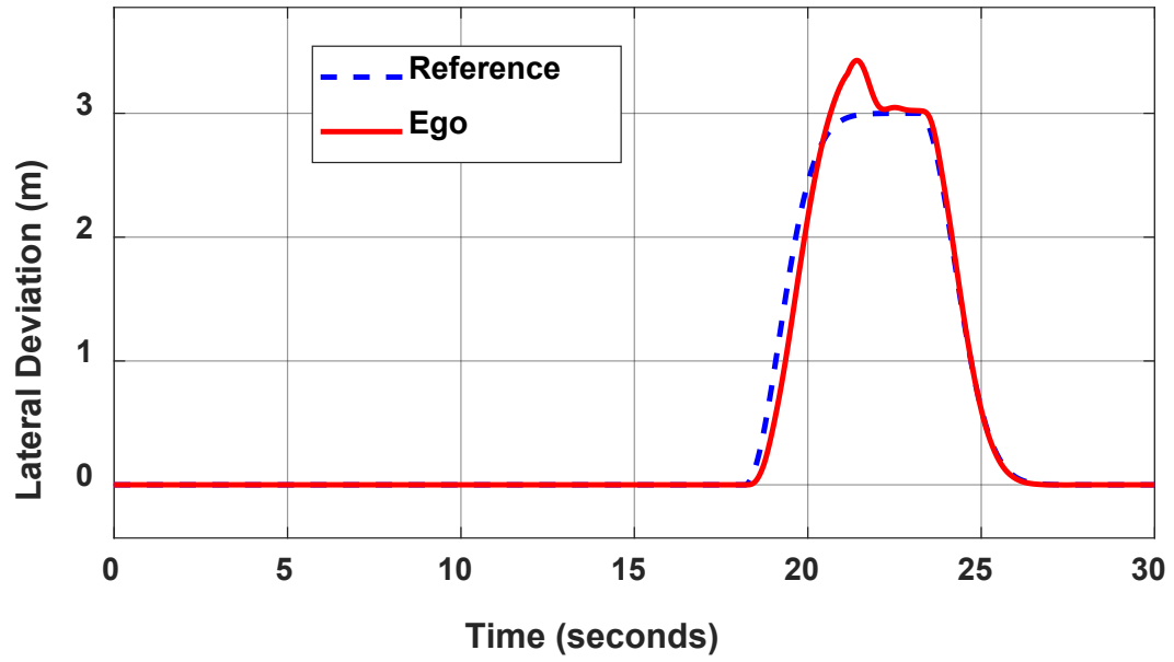
Figure 4.15: Comparison of the reference trajectory and actual vehicle trajectory obtained to avoid a collision
