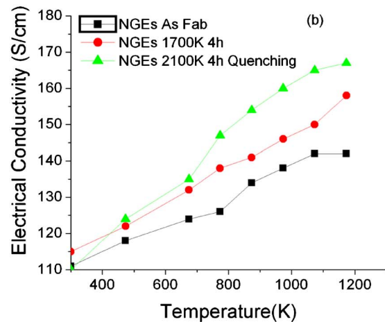
FIG. 5. (Color online) The dc electrical conductivities measured as a function of measuring temperatures for various (a) B:NGEs and (b) NGEs.
