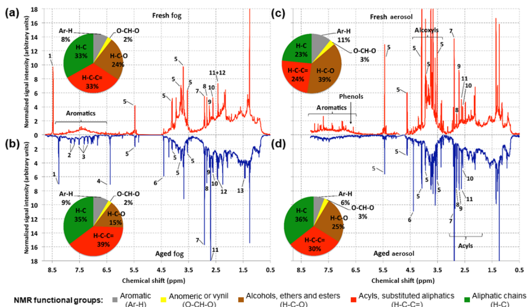
Figure 2. The ^1\text{H} -NMR spectra of selected fog water (a, b) and aerosol (c, d) samples, and their corresponding functional group distribution. A set of specific resonances was attributed to individual compounds: (1) formate, (2) phthalic acid, (3) ammonium, (4) maleic acid, (5) levoglucosan, (6) hydroxy-methanesulfonic acid, (7) trimethylamine, (8) methanesulfonic acid, (9) dimethylamine, (10) monomethylamine, (11) succinic acid, (12) pyruvic acid, and (13) lactic acid. The sample names fresh fog, aged fog, fresh aerosol, and aged aerosol correspond to SPC0106F, SPC0201F, BO0204N, and BO0213D, respectively.
