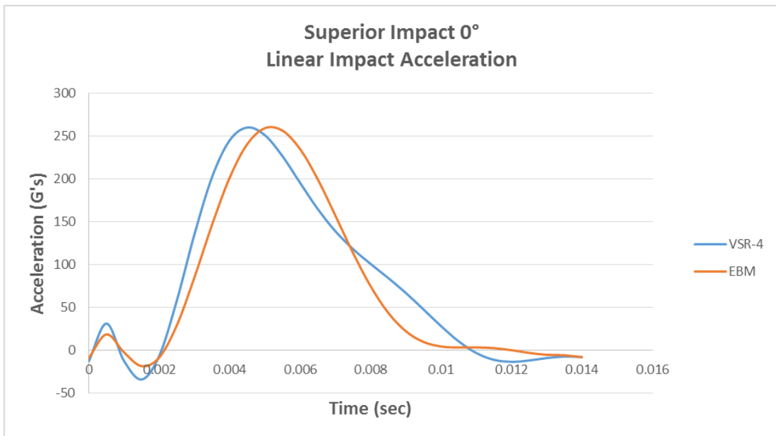
Figure 9-63 VSR4 and EBM Helmet – Superior Impact - Linear Acceleration
