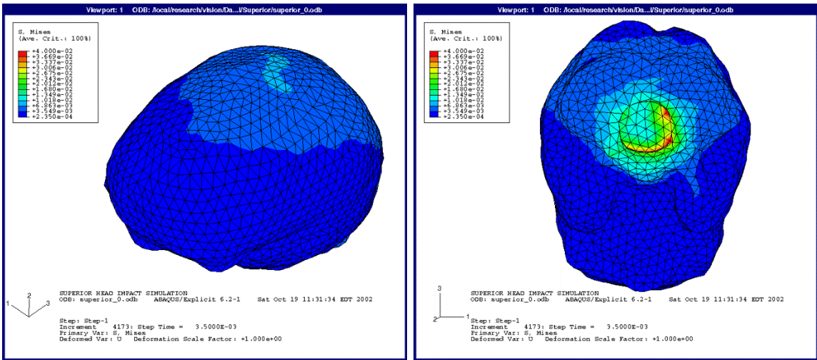
Figure 2-40 Superior Impact 0° - von Mises Stress Distribution
