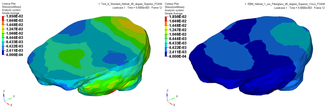
Figure 9-70 VSR4 (left) and EBM (right) Helmet - Superior Impact 45° - von Mises Stress
