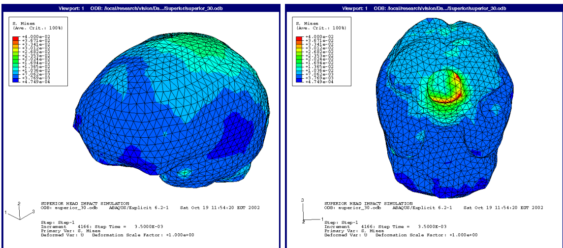
Figure 2-44 Superior Impact 30° - von Mises Stress Distribution
